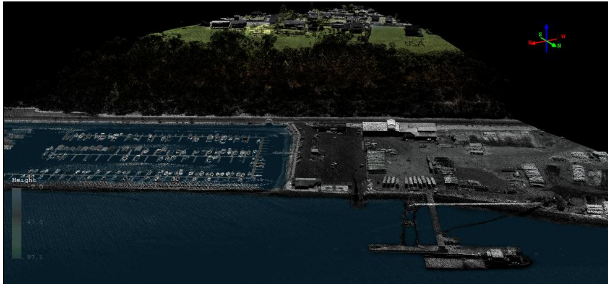
Figure 15. The image is looking inland at a marina SE of the Hill St. & Marine Dr. junction, Port Angeles, WA. The image is a 3D point cloud colored by height and intensity.
