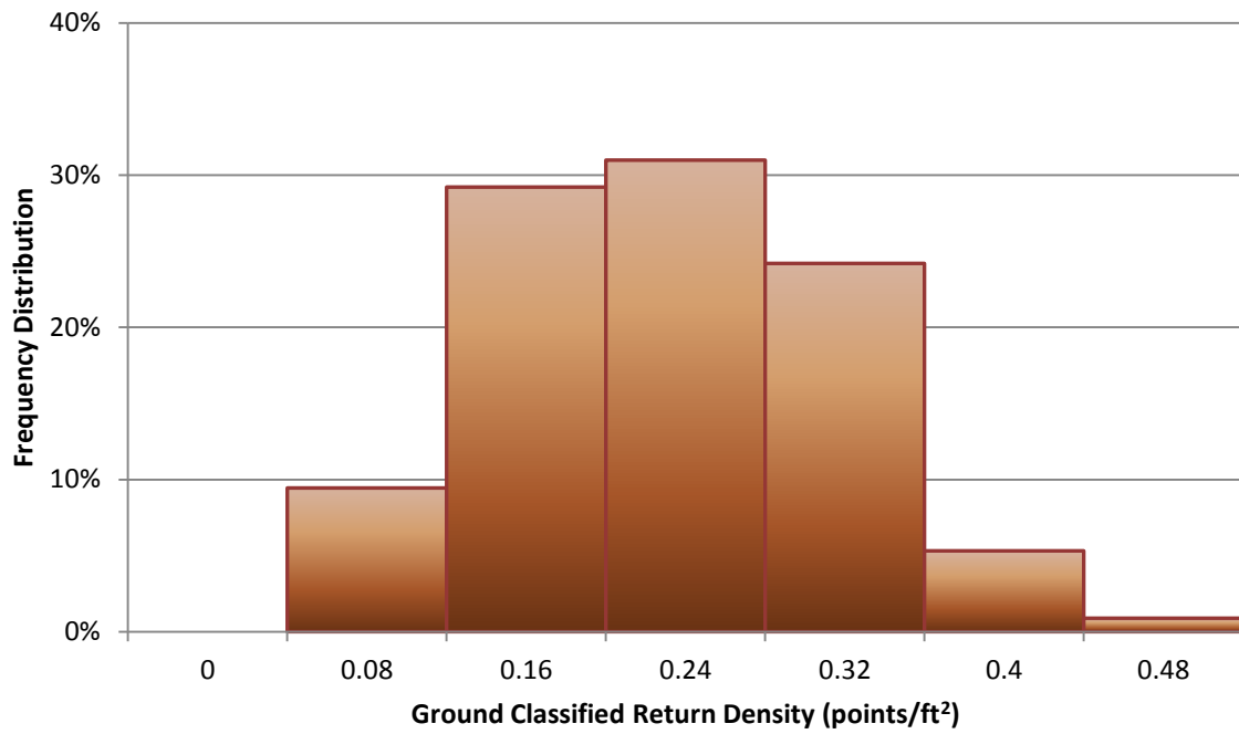
Figure 5. Density distribution for ground classified laser points.
