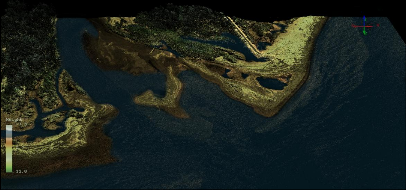
Figure 13. The image is looking southwest at the mouth of the Elwha River, WA. The image is a 3D point cloud colored by height and intensity.
