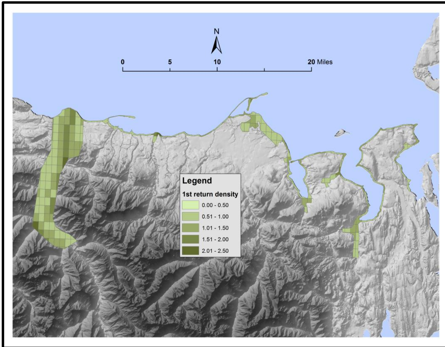
Figure 6. First Return density by 1/100 th USGS tile (points/ft 2 ).
