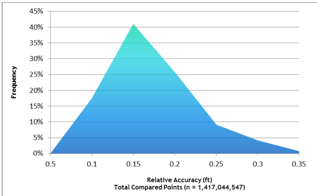
Figure 8. Distribution of relative accuracies per flight line, non-slope-adjusted.
