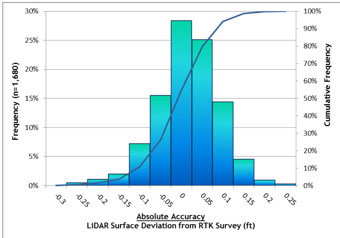
Figure 9. Absolute Accuracy - Histogram Statistics.
