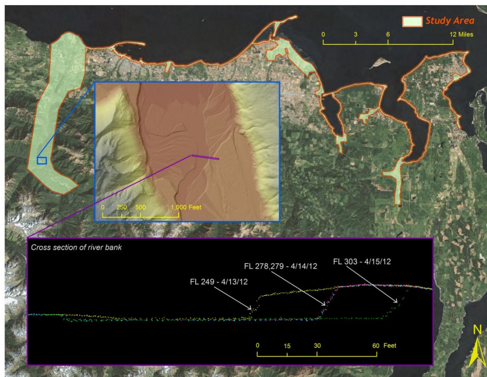
Figure 10. Illustration of sediment erosion along the Elwha River, the cross section shows LiDAR returns (labeled by flight line and acquisition date) of the stream bank over a three day period.
