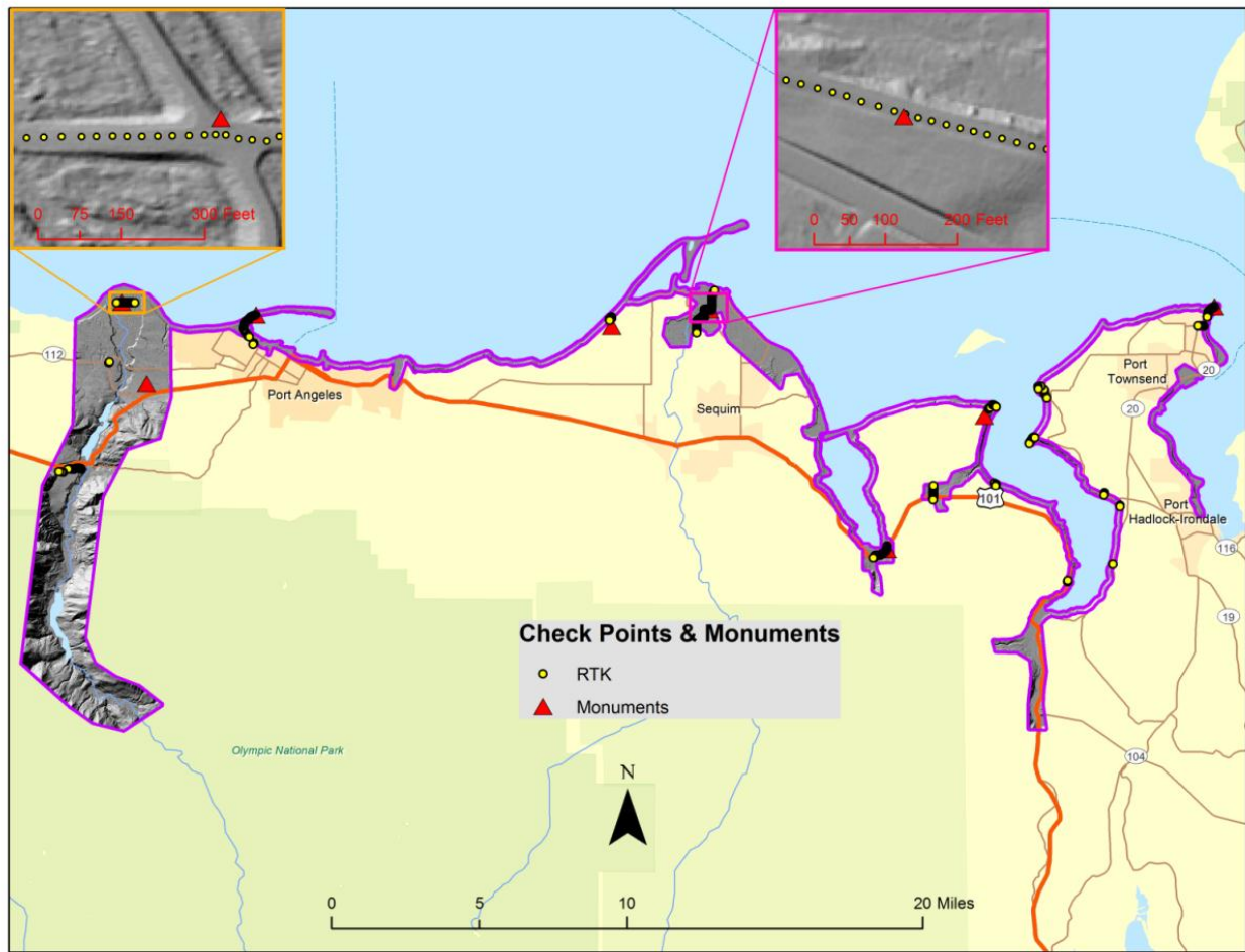
Figure 3. RTK check point (1,680) and control monument (8) locations used in the Jefferson/Clallam AOI.
