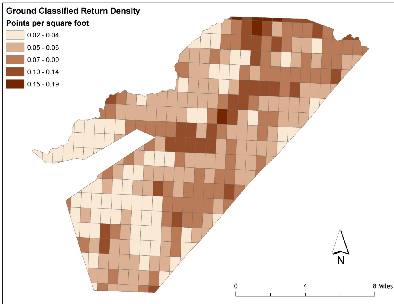
Figure 6. Ground density by 1/100 th USGS tile
