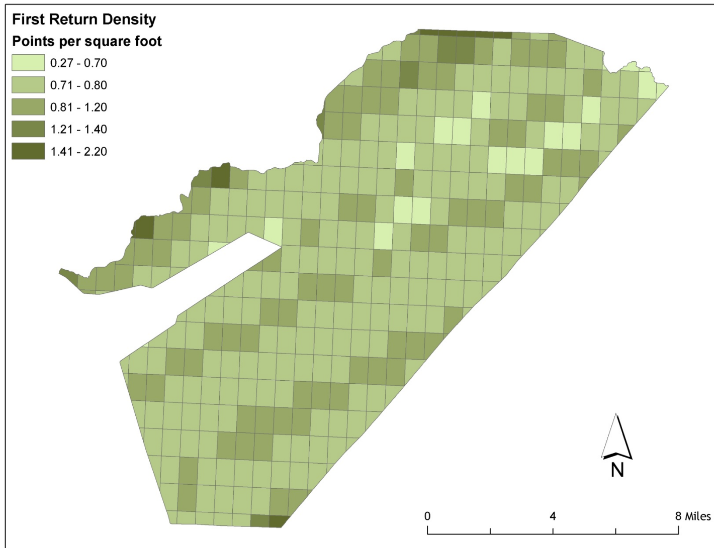
Figure 5. First return density by 1/100 th USGS tile.
