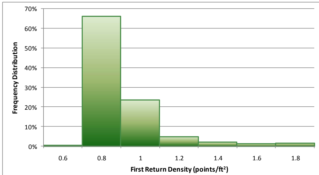
Figure 3. Density distribution for first return laser points
