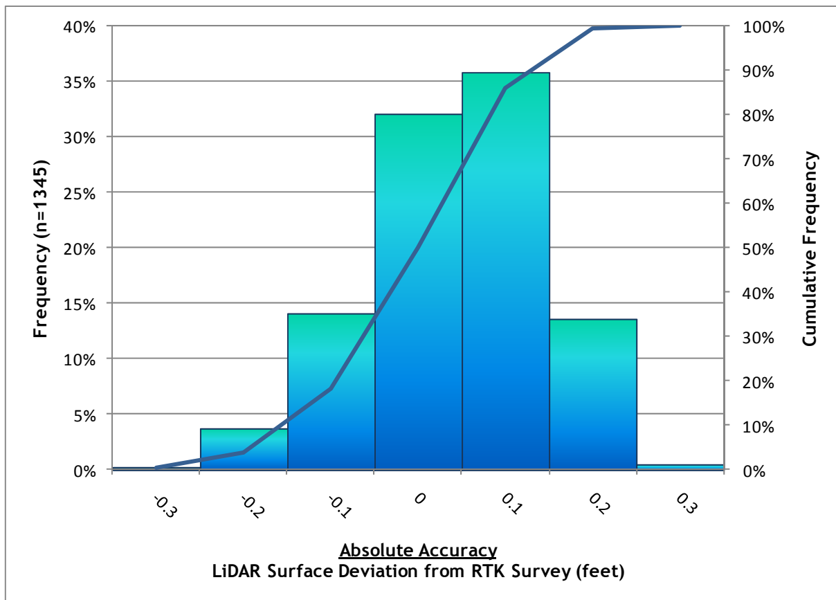
Figure 8. Absolute Accuracy - Histogram Statistics.
