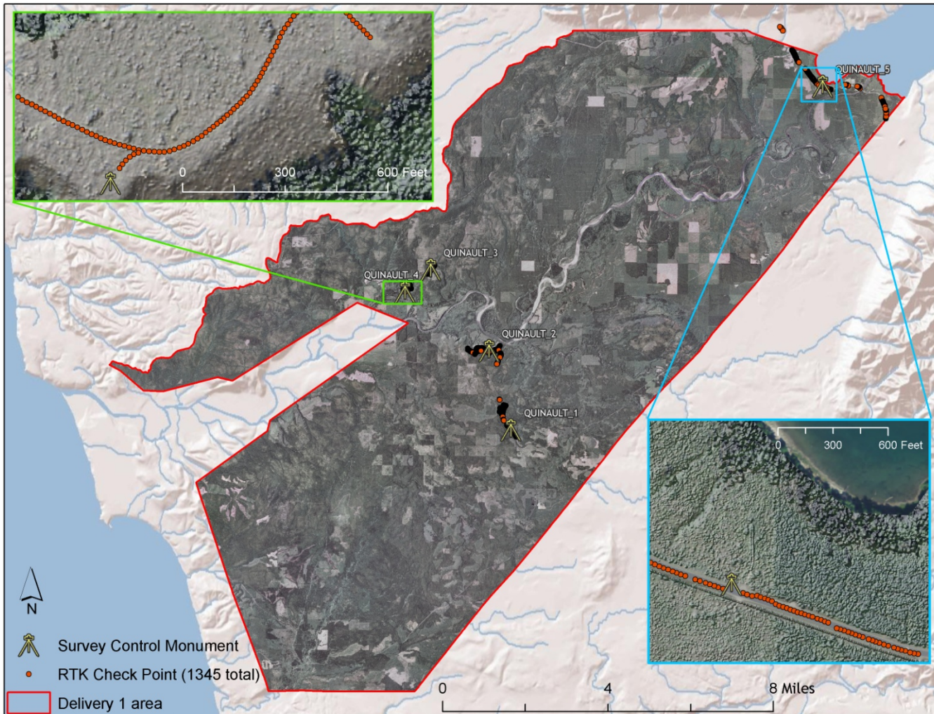
Figure 2. RTK check point and control monument locations used in the Quinault River Basin survey area
