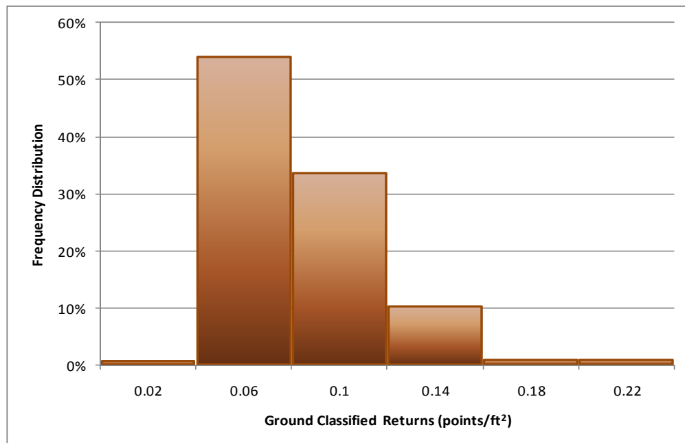
Figure 4. Density distribution for ground classified laser points
