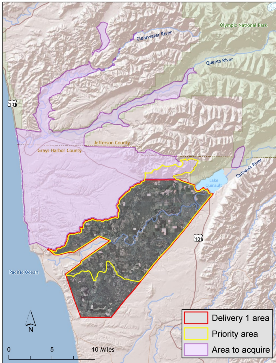
Figure 1. Quinault River Basin area of interest, Washington.
