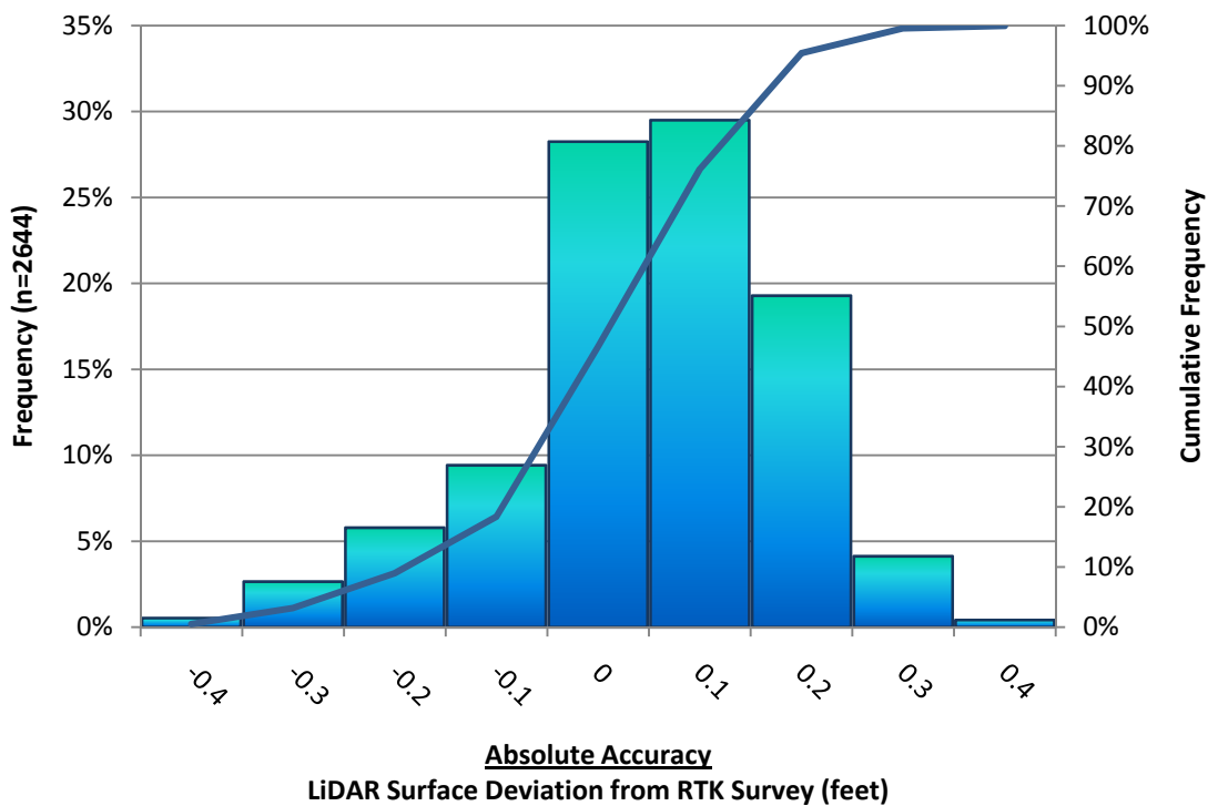
Figure 10. Absolute Accuracy - Histogram Statistics, based on hard surface points
