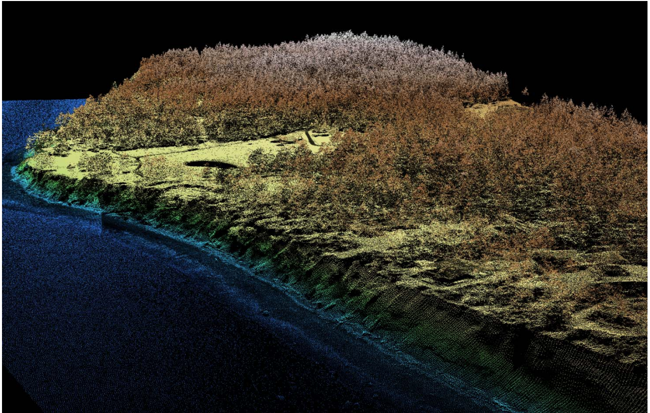
Figure 17. Point cloud image derived from LiDAR data. Looking northeast along the Middle Channel into Griffin Bay on the western coastline of Lopez Island.
