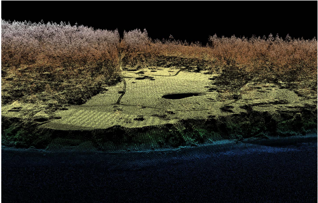
Figure 18. Point cloud image derived from LiDAR data. Looking east on the western coastline of Lopez Island along Kings Point Road from the Middle Channel.
