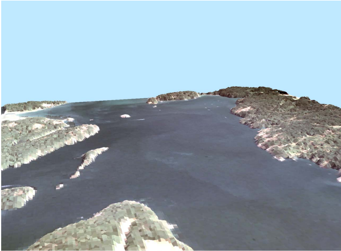
Figure 16. Highest hit LiDAR data with NAIP imagery draped over the model. Looking southwest from Center Island across Lopez Sound to Lopez Island.
