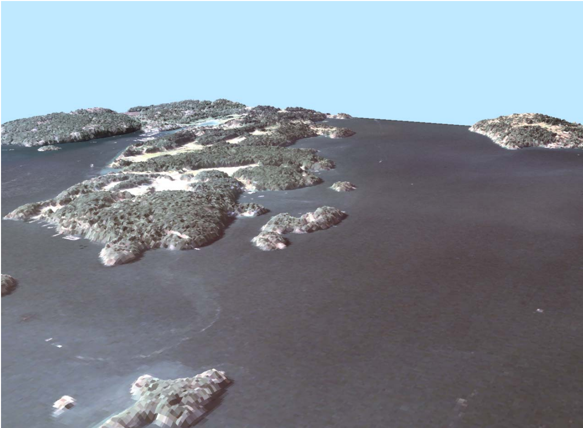
Figure 15. Highest hit LiDAR data with NAIP imagery draped over the model. Looking northeast along the shoreline of Orcas Island. Deer harbor is in the background.
