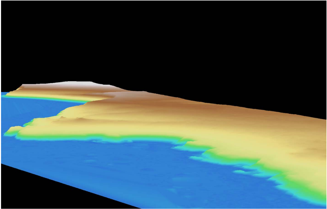
Figure 19. Bare-earth image derived from ground classified points and colored by elevation. Looking north along western side of Lopez Island on Griffin Bay.
