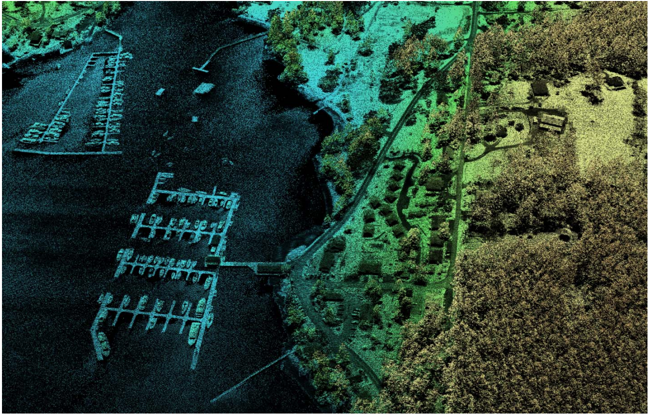
Figure 13. Point cloud image derived from LiDAR data. Looking north over Deer Harbor and Deer Harbor Road along the San Juan Channel on Orcas Island.
