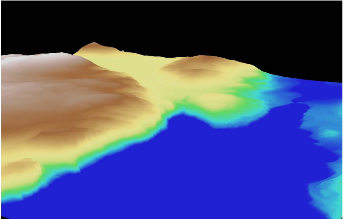
Figure 14. Bare-earth image derived from ground classified points that is colored by elevation. Looking northwest over Deer Harbor with a view of Orcas Island in the background.
