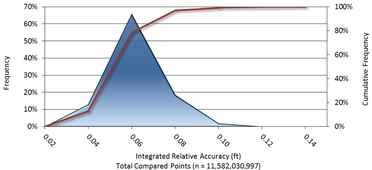
Figure 14: Frequency plot for relative vertical accuracy between flight lines
