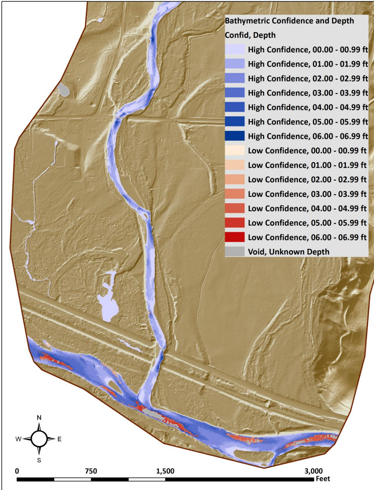
Figure 5: Sample image from the Teanaway Streams Topobathymetric project showing confidence values and data voids
