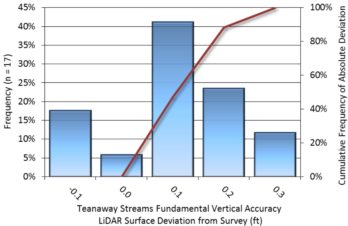
Figure 11: Frequency histogram for LiDAR surface deviation from ground check point values
