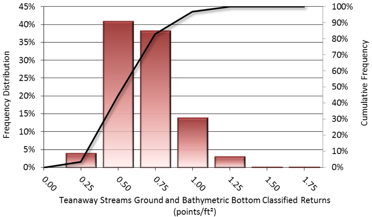
Figure 8: Frequency distribution of ground return densities per 300 x 300 ft cell
