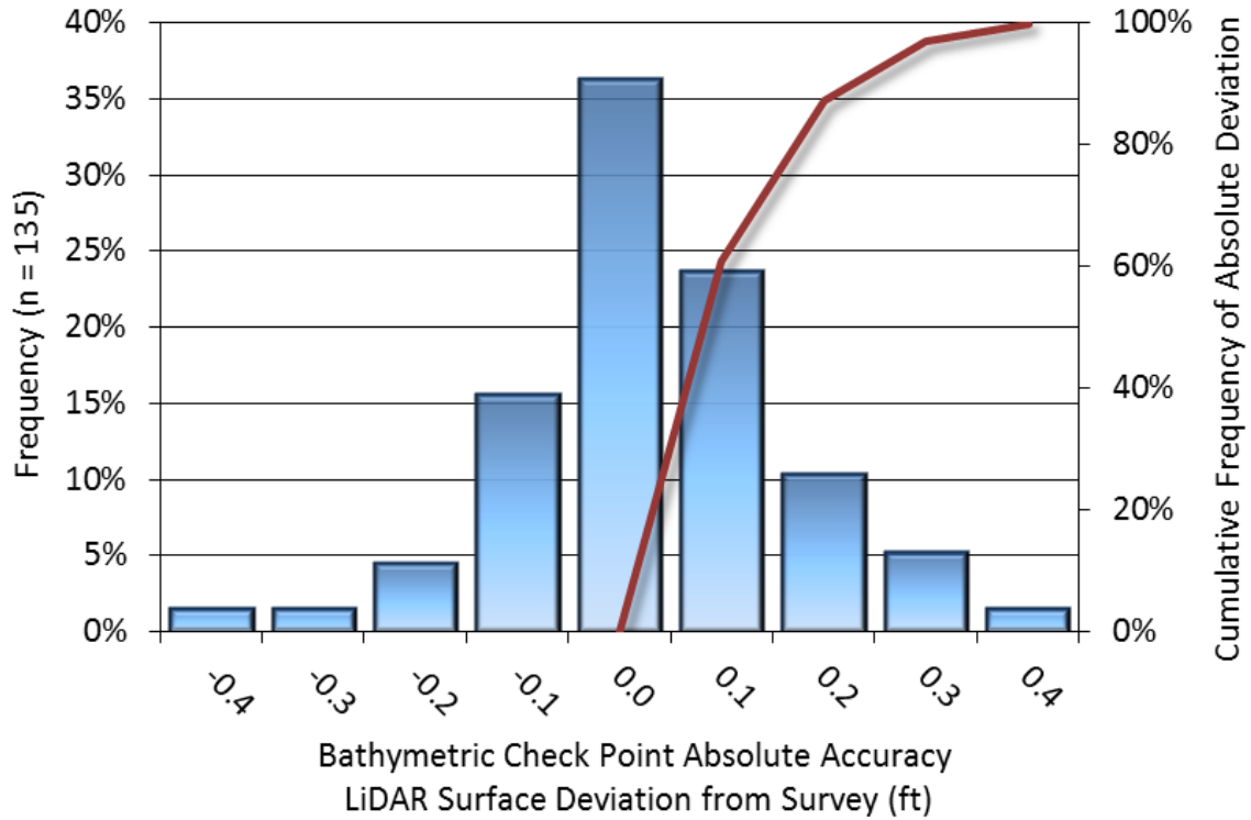
Figure 12: Frequency histogram for LiDAR surface deviation from bathymetric check point values
