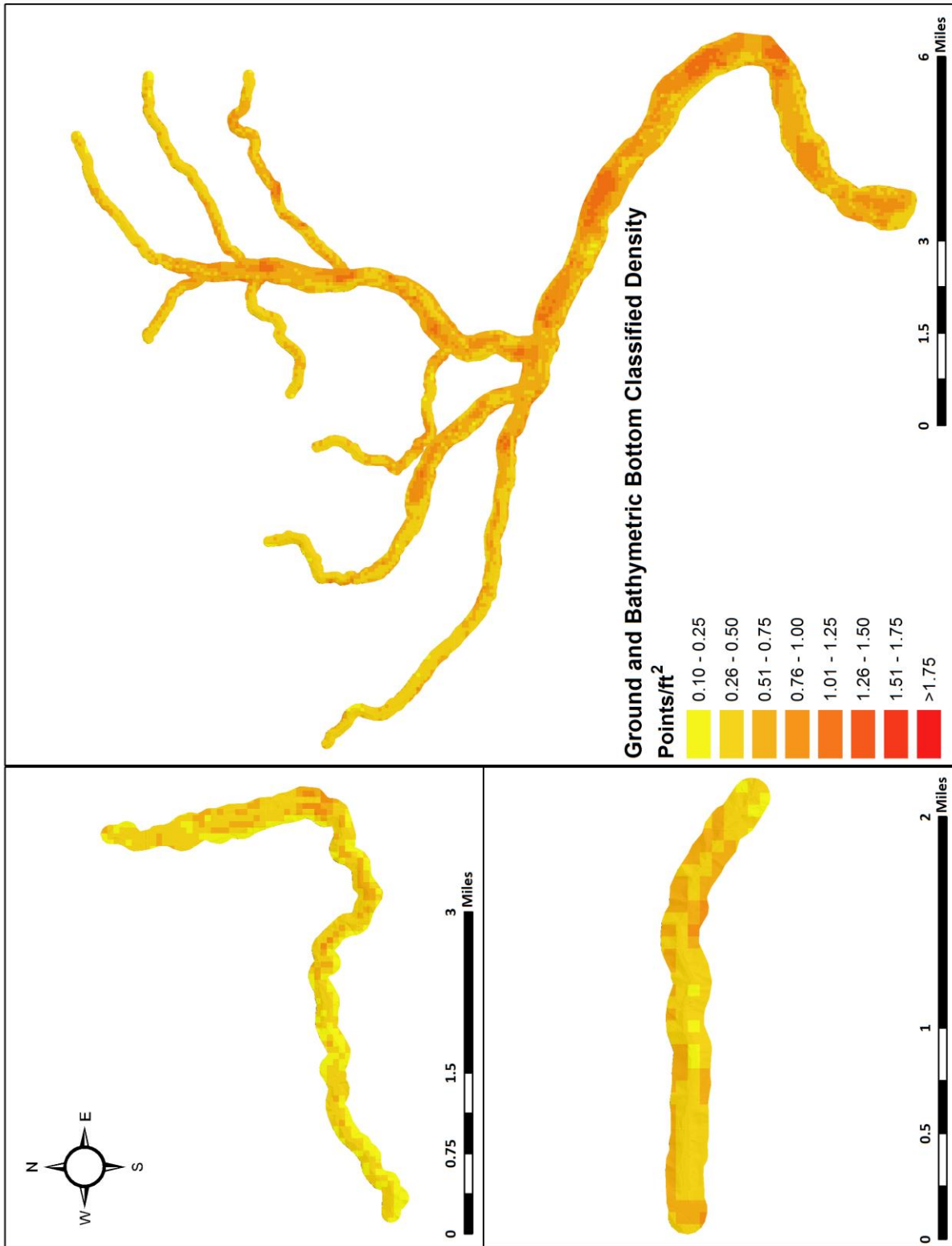
Figure 10: Ground and bathymetric bottom classified density map for the Teanaway Streams site (300 ft x 300 ft cells)
