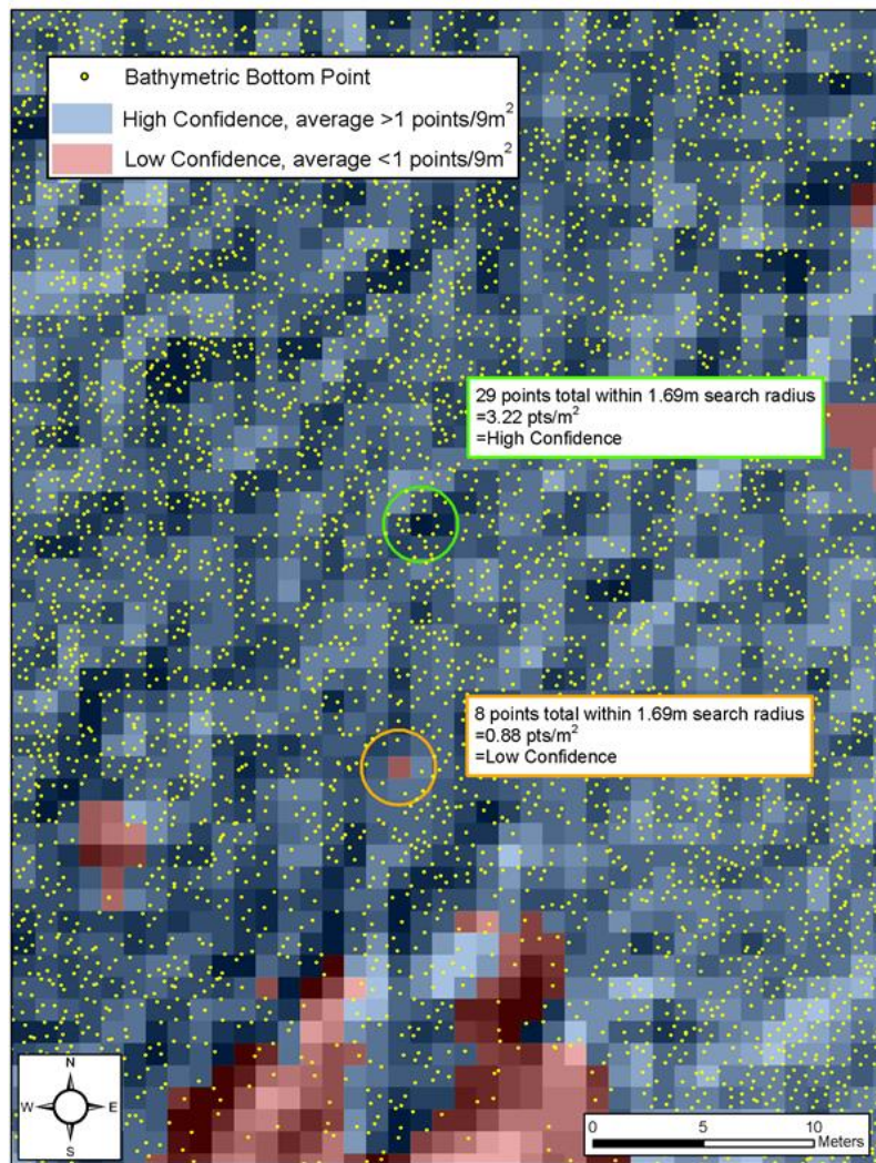
Figure 4: Sample plot of low and high confidence in bathymetric returns
