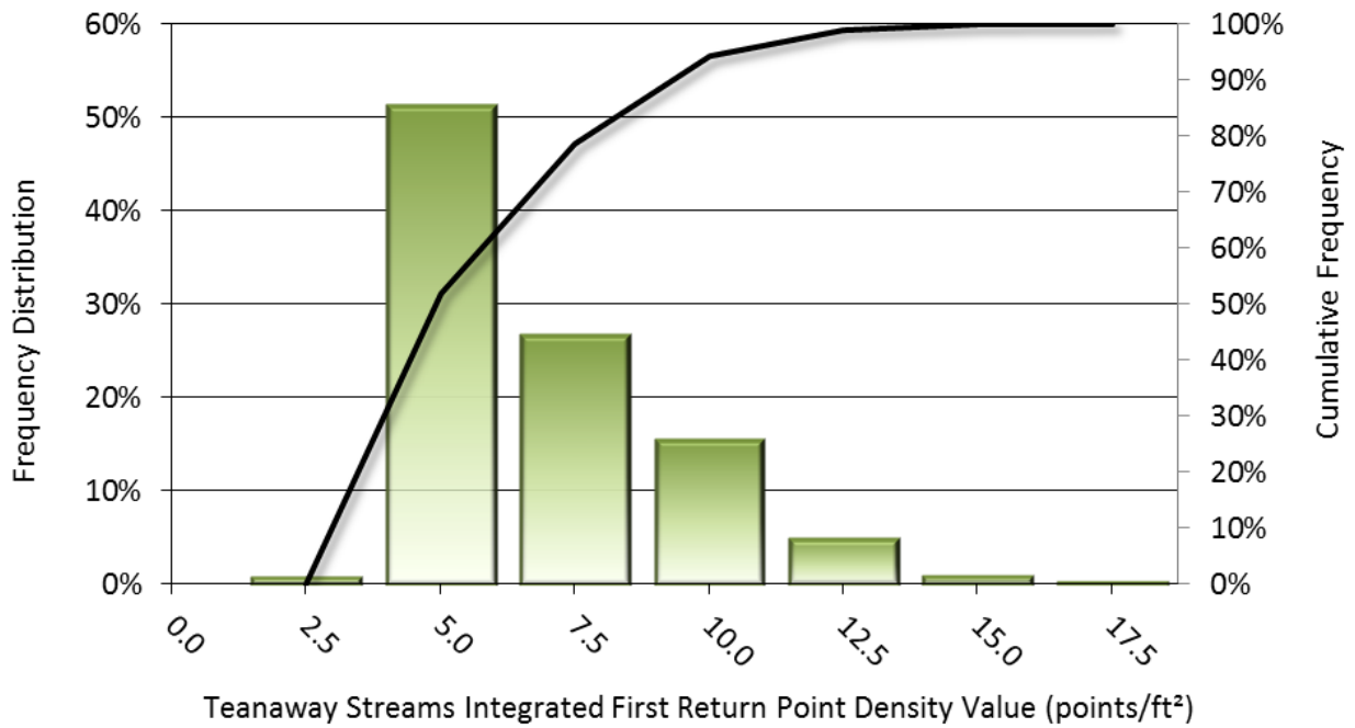
Figure 7: Frequency distribution of first return densities per 300 x 300 ft cell
