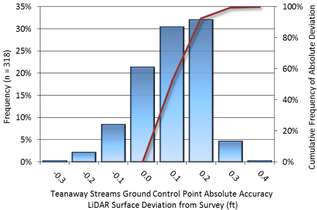
Figure 13: Frequency histogram for LiDAR surface deviation from ground control point values
