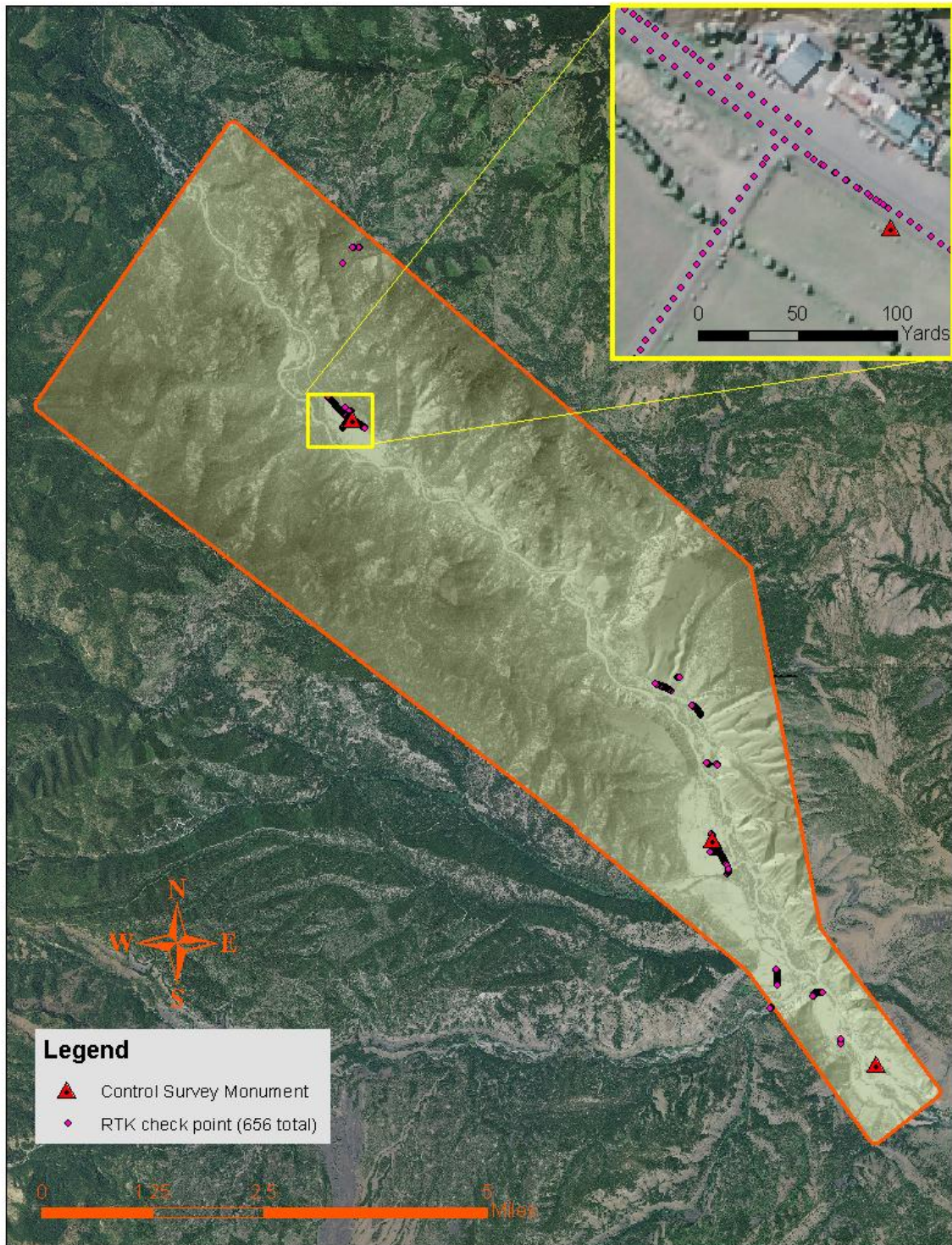
Figure 2. RTK check point (656) and control monument (3) locations used in the Upper Naches River and Nile Slide AOI.
