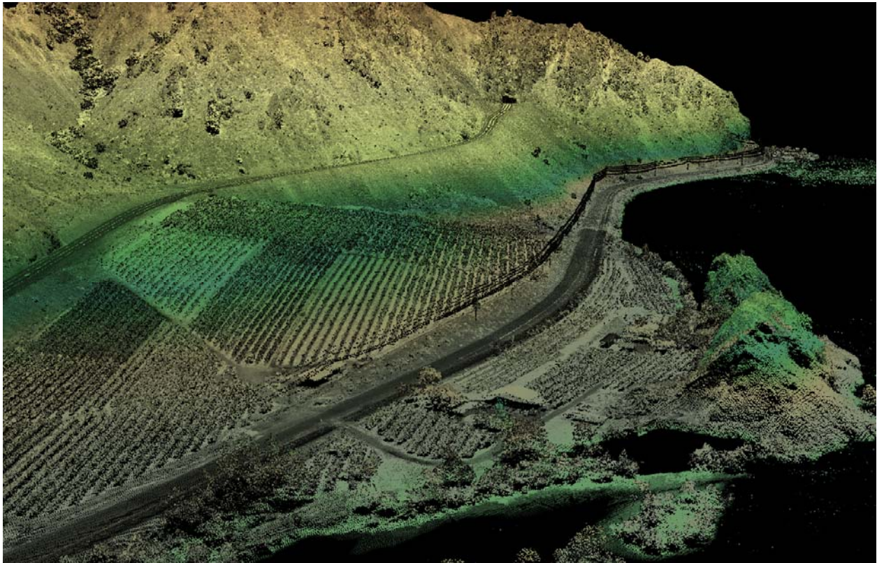
Figure 13. LiDAR derived point cloud image colored by elevation textured by intensity. Looking uphill toward Hwy 97 Alt. toward tunnel at the junction with Hwy 97 (Columbia River on extreme right).
