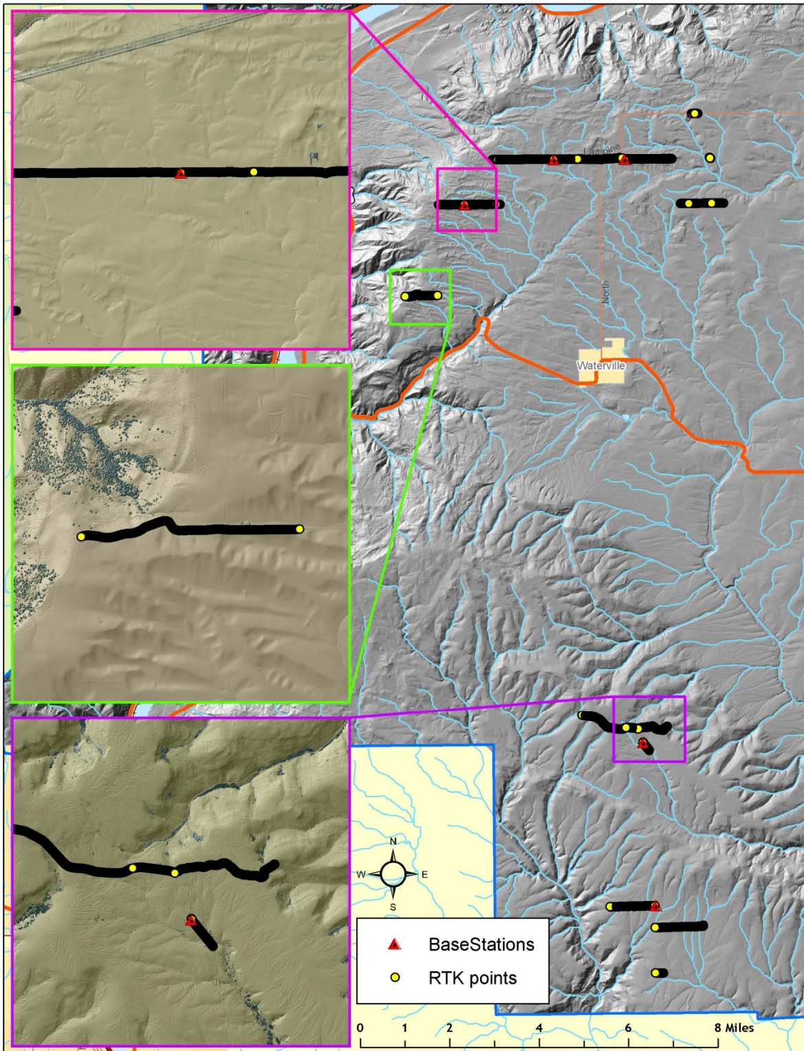
Figure 2. RTK and base station locations used for the Wenatchee USGS AOI. Image created from 3-ft LiDAR derived highest hit model over ESRI background data.
