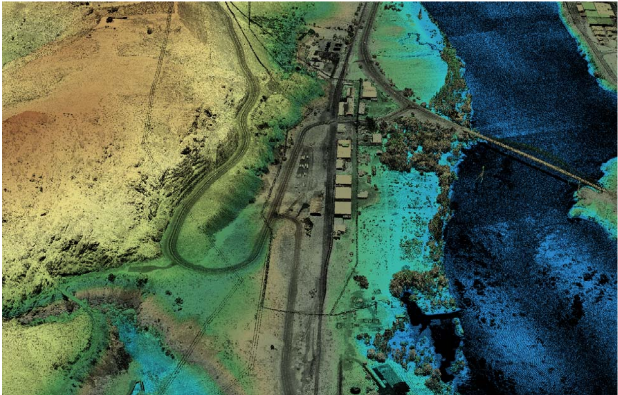
Figure 15. LiDAR derived point cloud image colored by elevation textured by intensity. Upstream view of the Columbia River (Lake Entiat) and Chelan Station, with Chelan Falls in the lower left corner of image.
