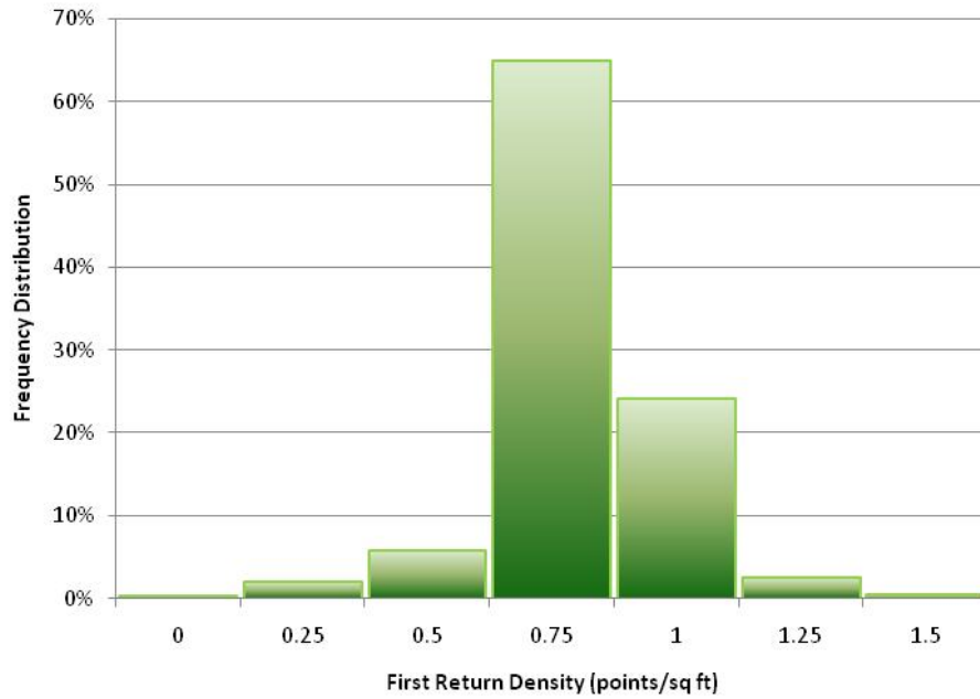
Figure 3. Density distribution for first return laser points
