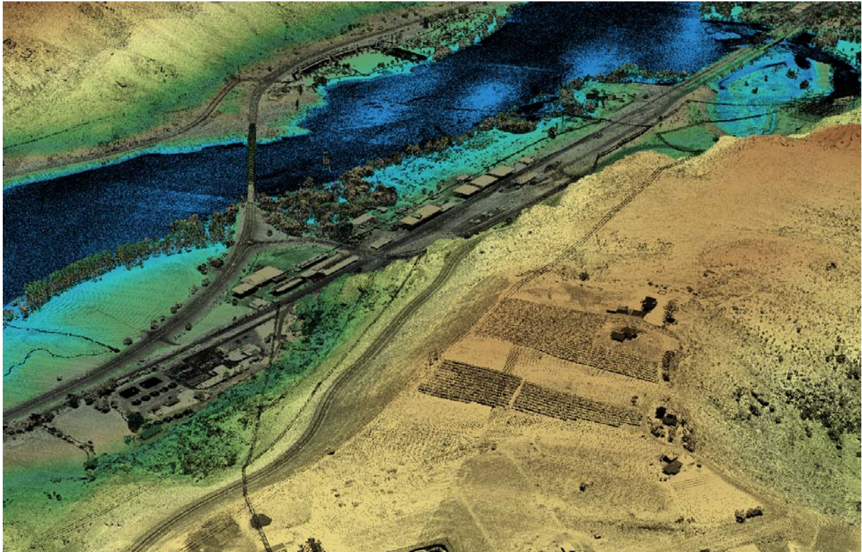
Figure 14. LiDAR derived point cloud image colored by elevation textured by intensity. Southeast view of Hwy 97 Columbia River crossing at Chelan Station.
