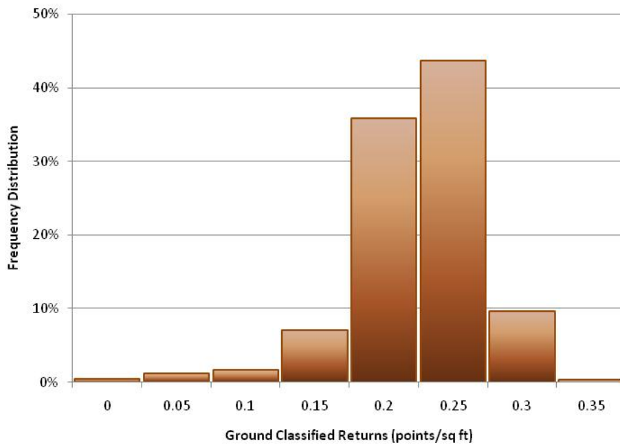
Figure 4. Density distribution for ground-classified laser points.
