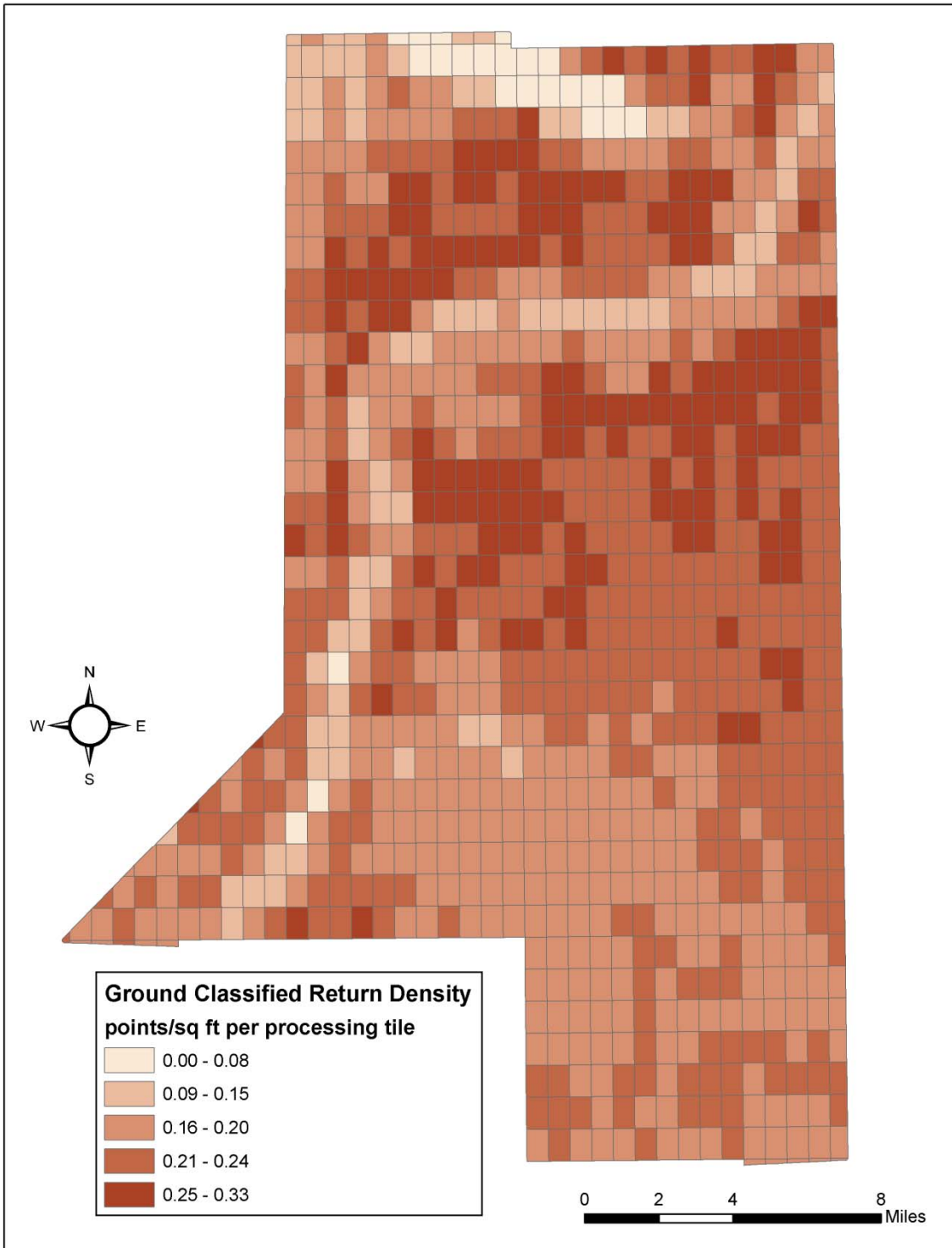
Figure 6. Ground-classified laser point data density per USGS 1/100th quadrangle
