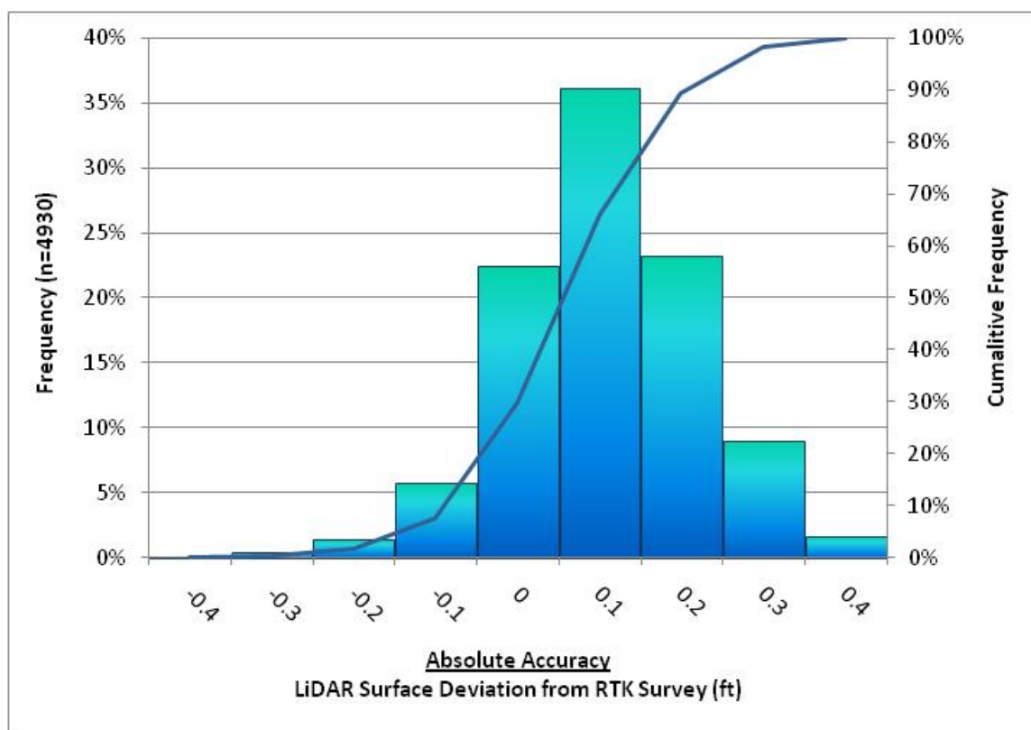
Figure 8. Absolute Accuracy - Histogram Statistics, based on hard surface points
